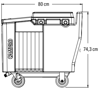
ICS125LB (带易滑轮)
