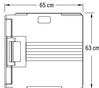
侧视图 UPC400
