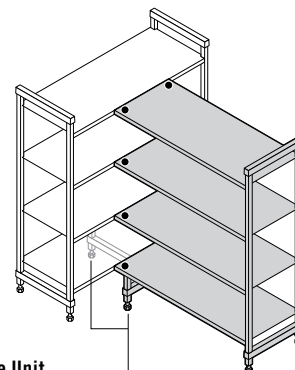
Starter unit + Add-on unit using 1 set of corner connectors per shelf and 2 dunnage stands.
