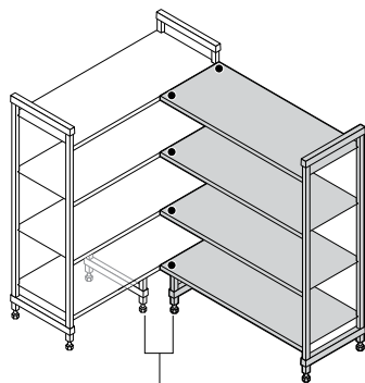
Starter Unit + Add-On Unit using 1 set of Corner Connectors per shelf and 2 Dunnage Stands. —
